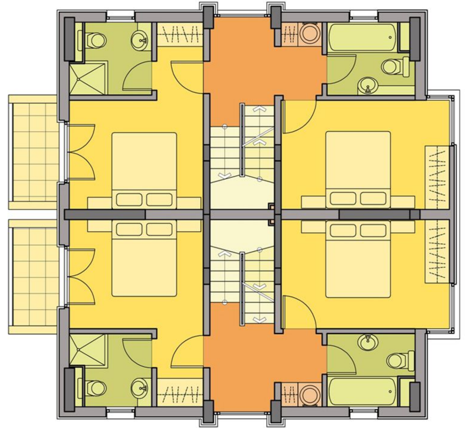
Second Floor
