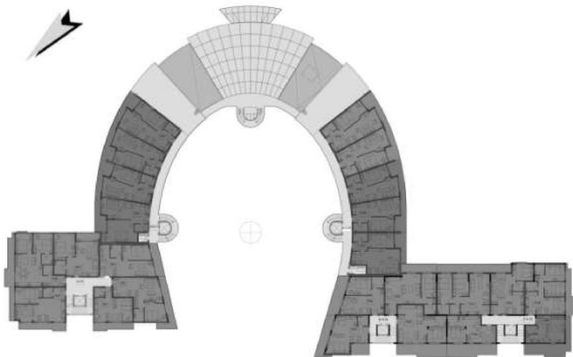
THIRD FLOOR
