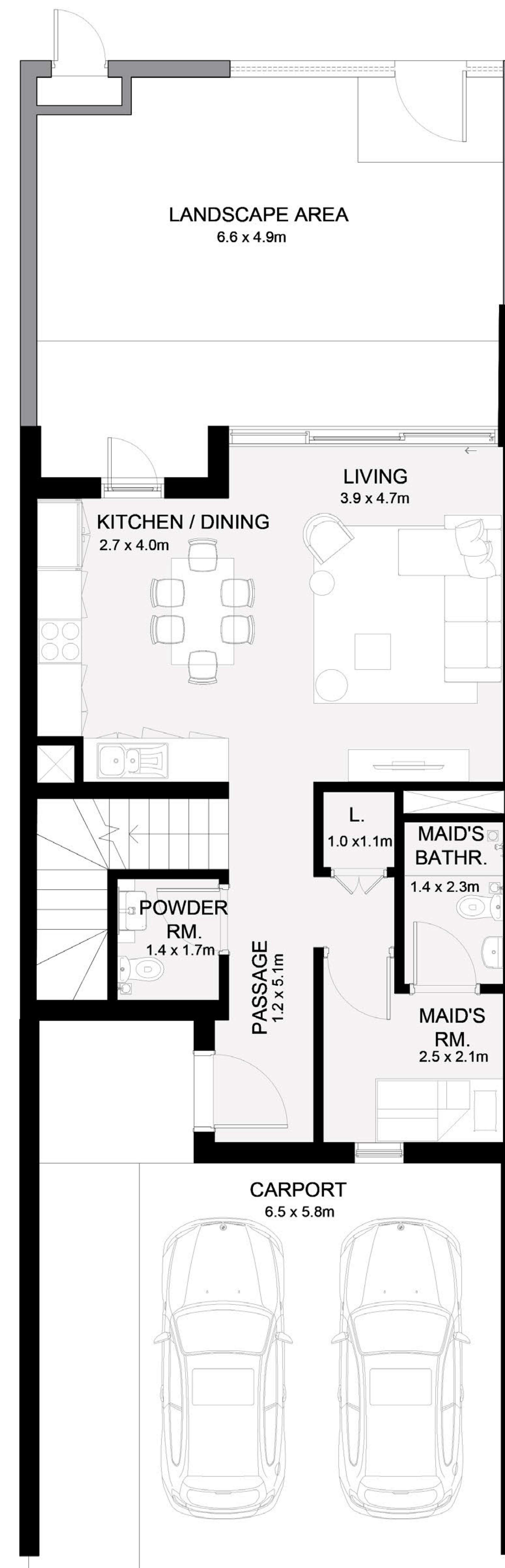
GROUND FLOOR
