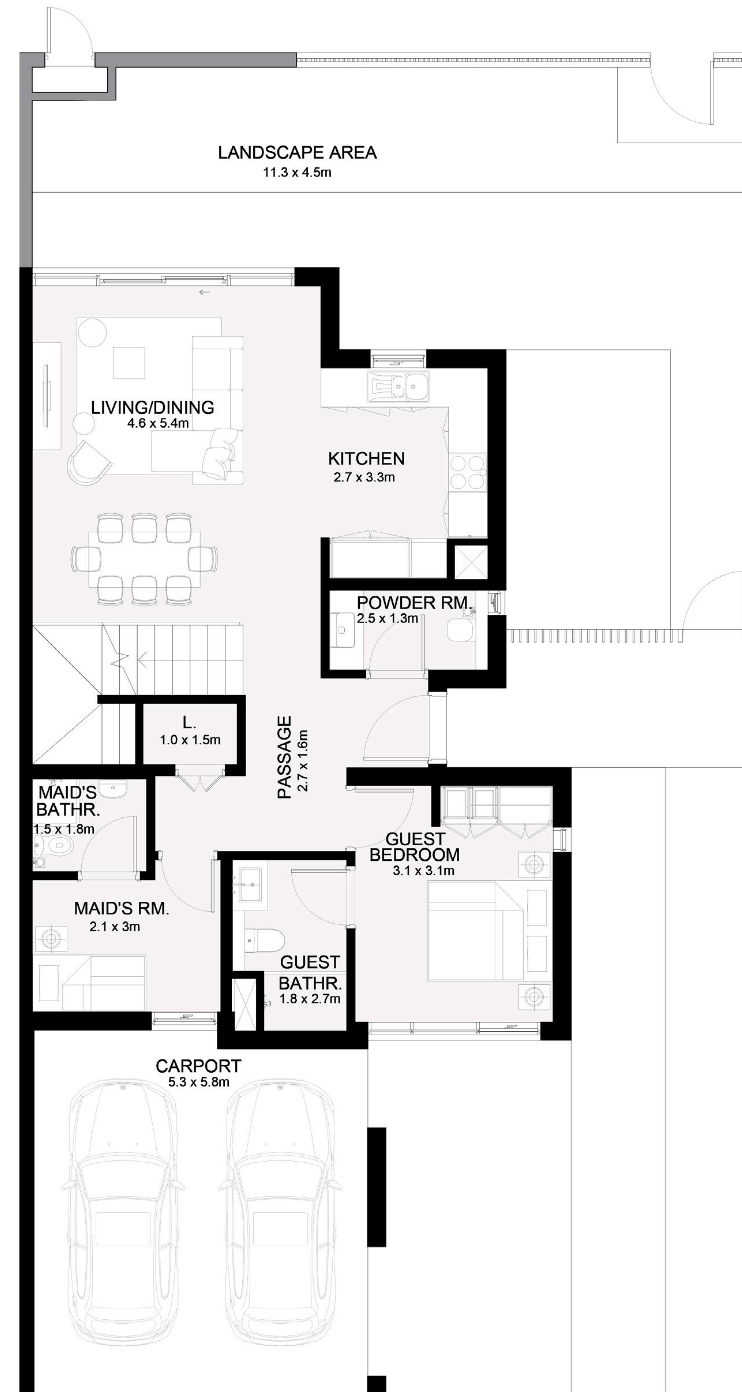
GROUND FLOOR
