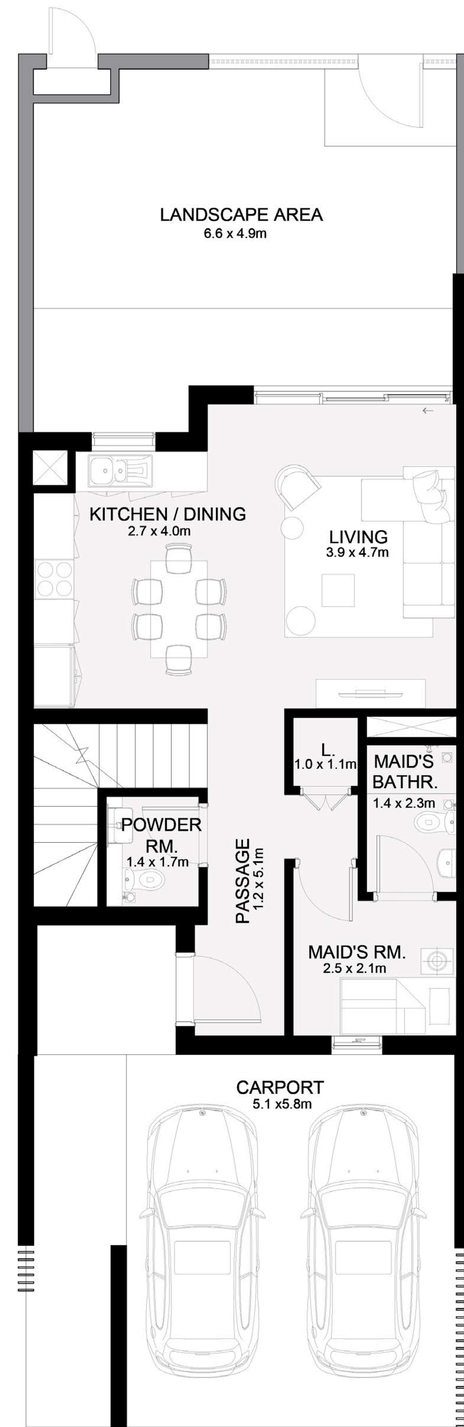
GROUND FLOOR
