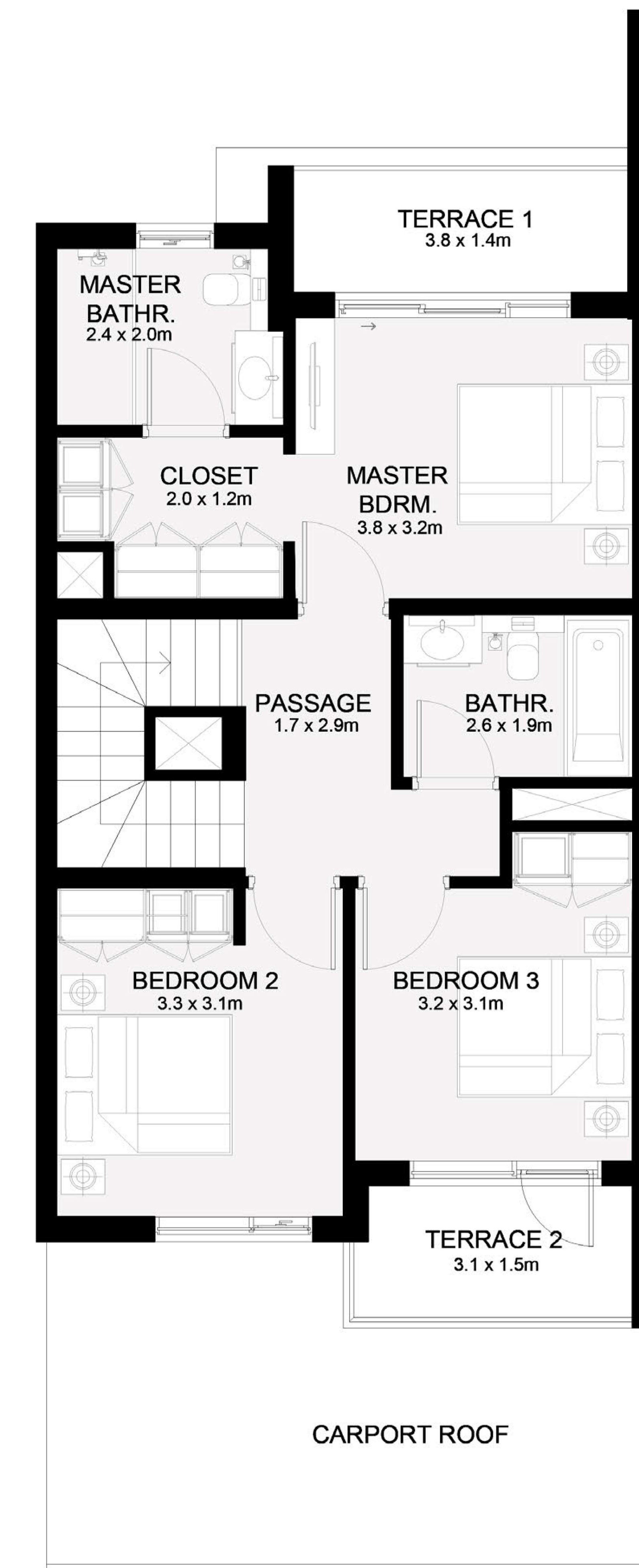
FIRST FLOOR
