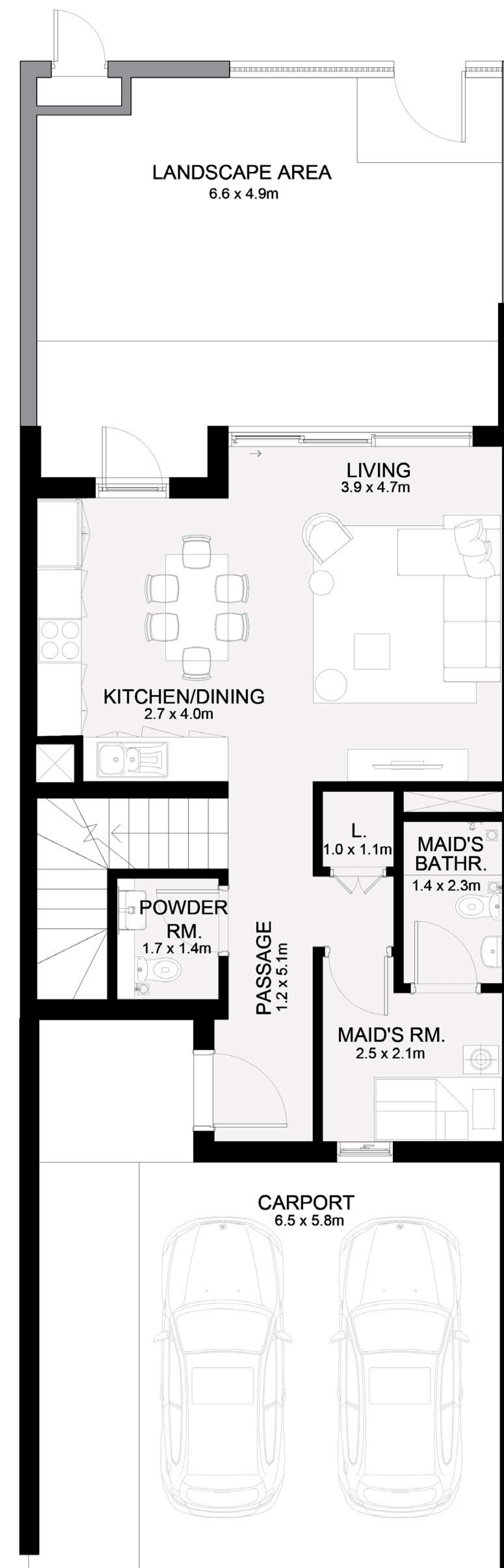
GROUND FLOOR
