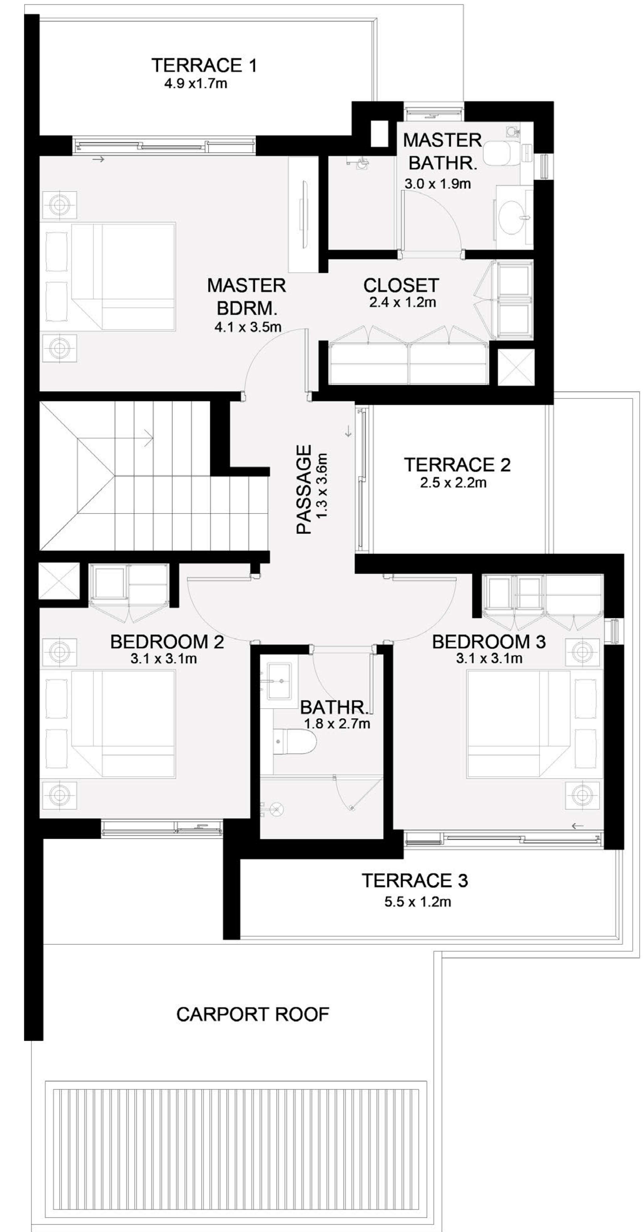
FIRST FLOOR
