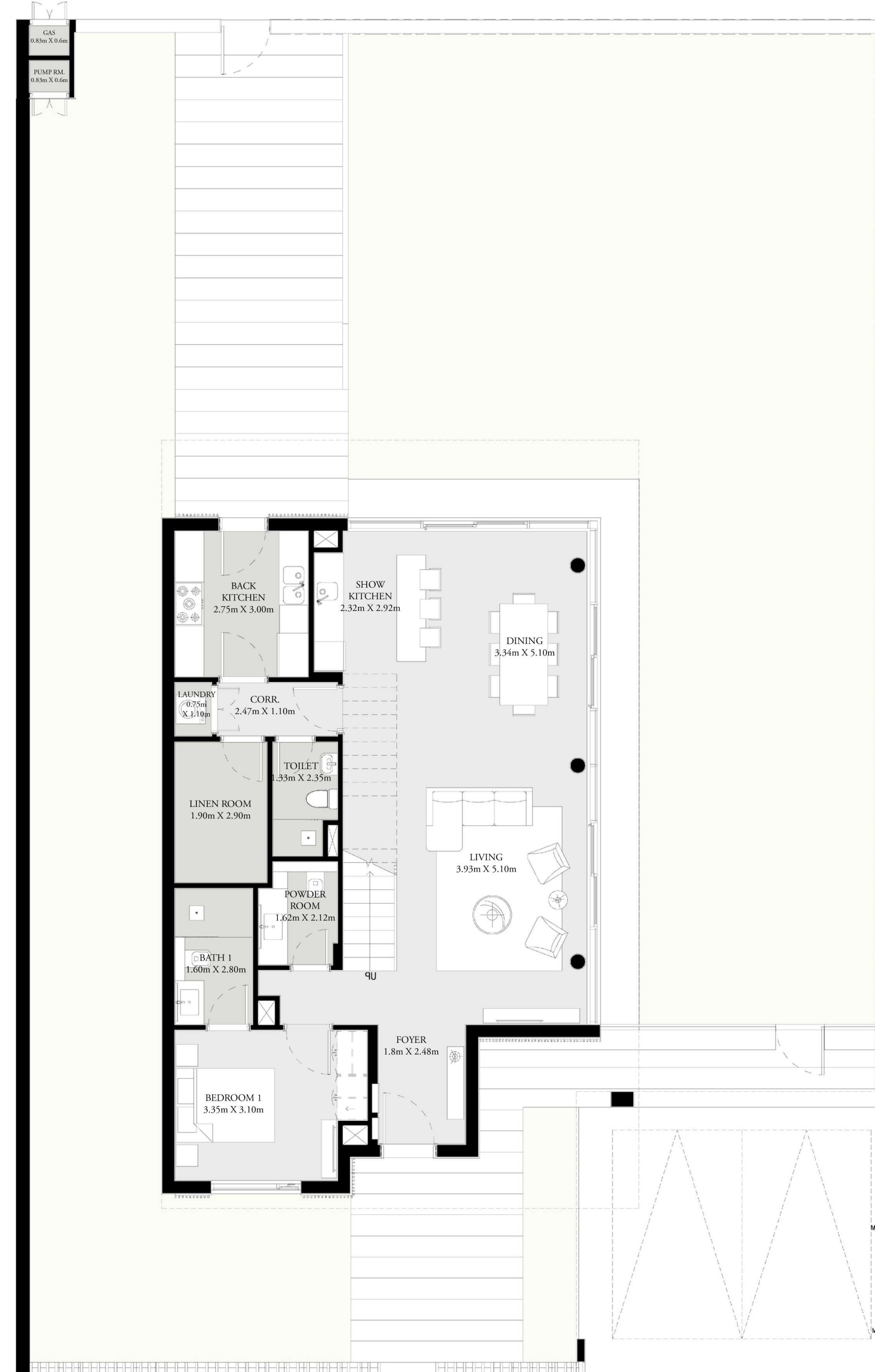
GROUND FLOOR
