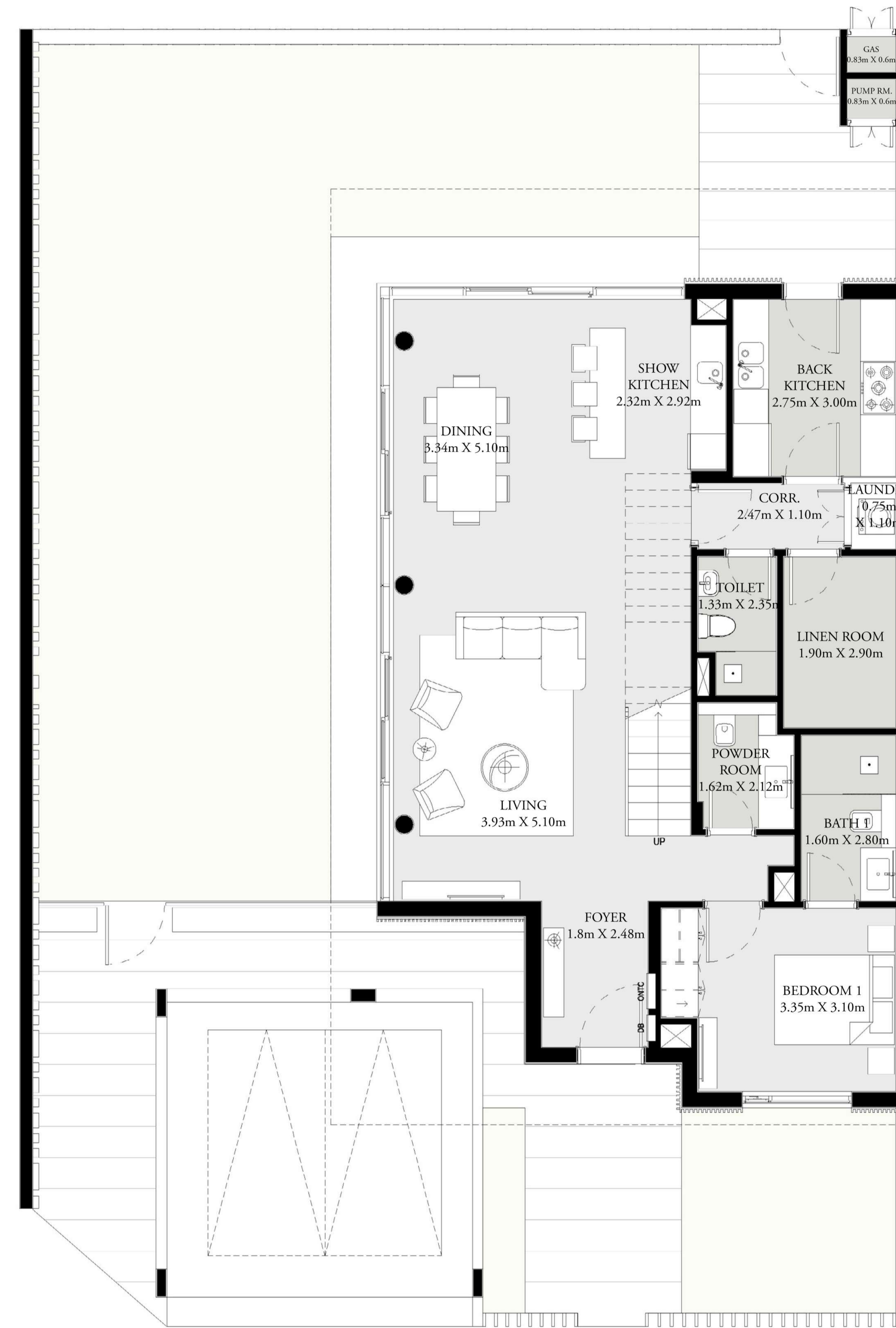
GROUND FLOOR
