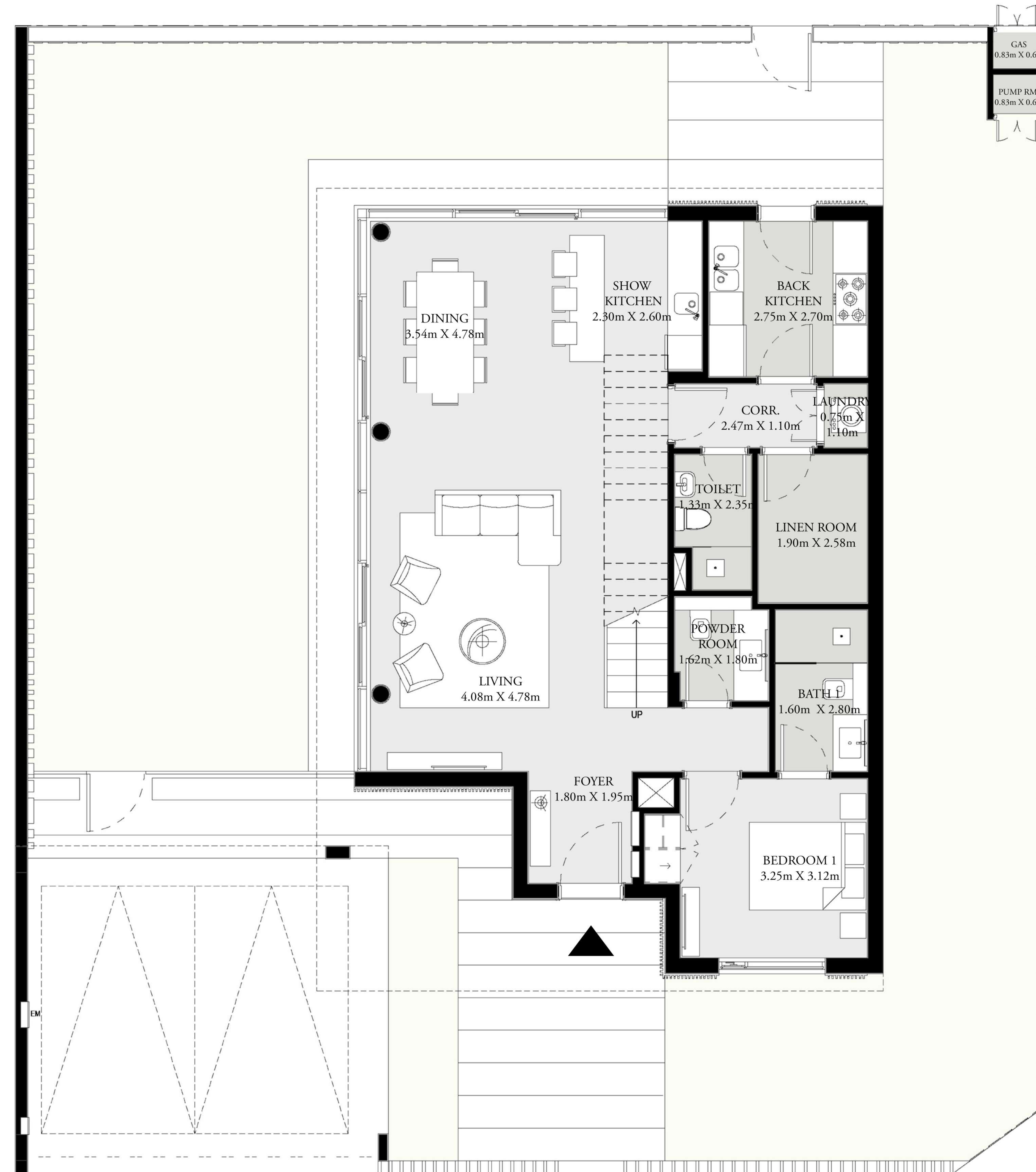
GROUND FLOOR
