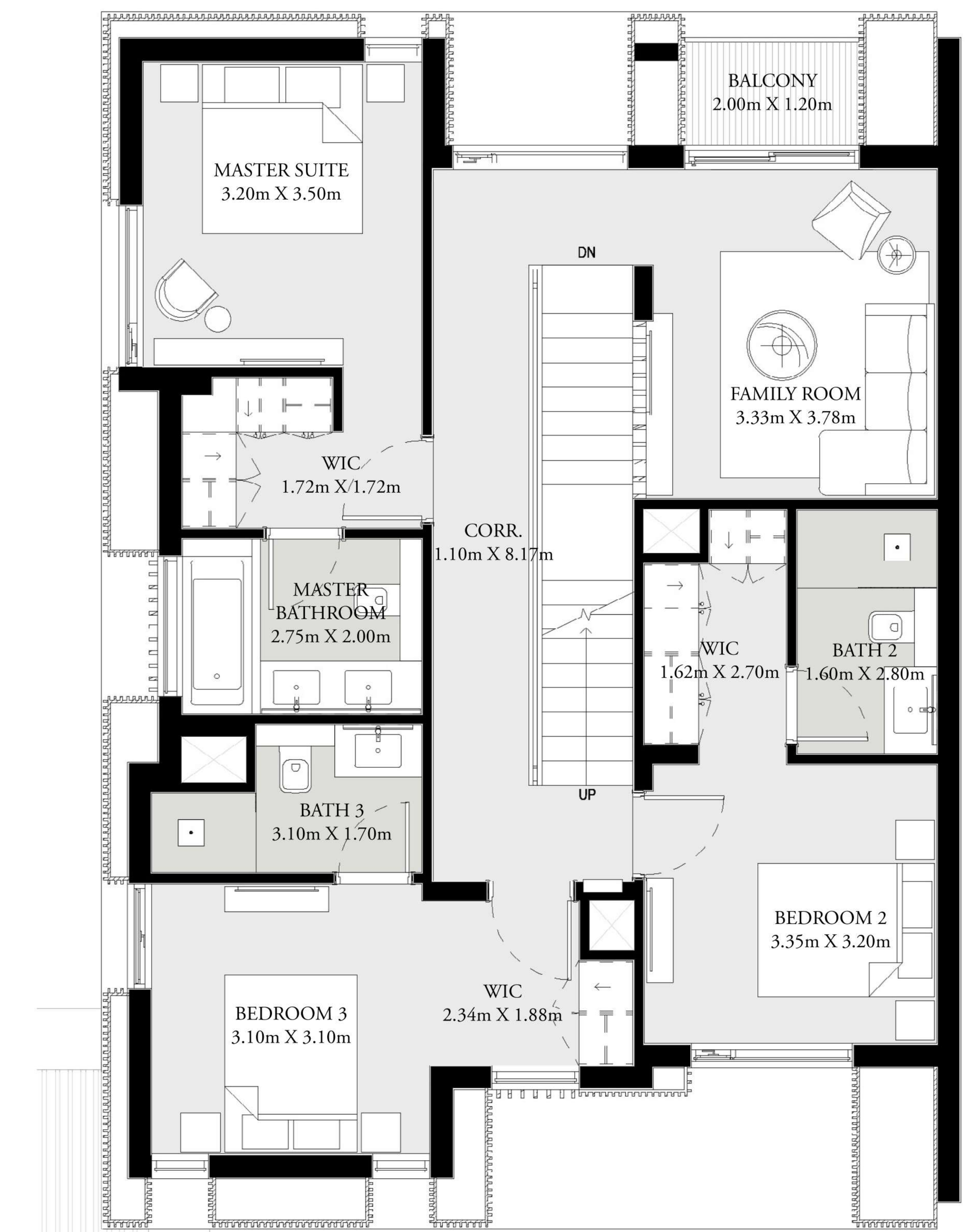
FIRST FLOOR
