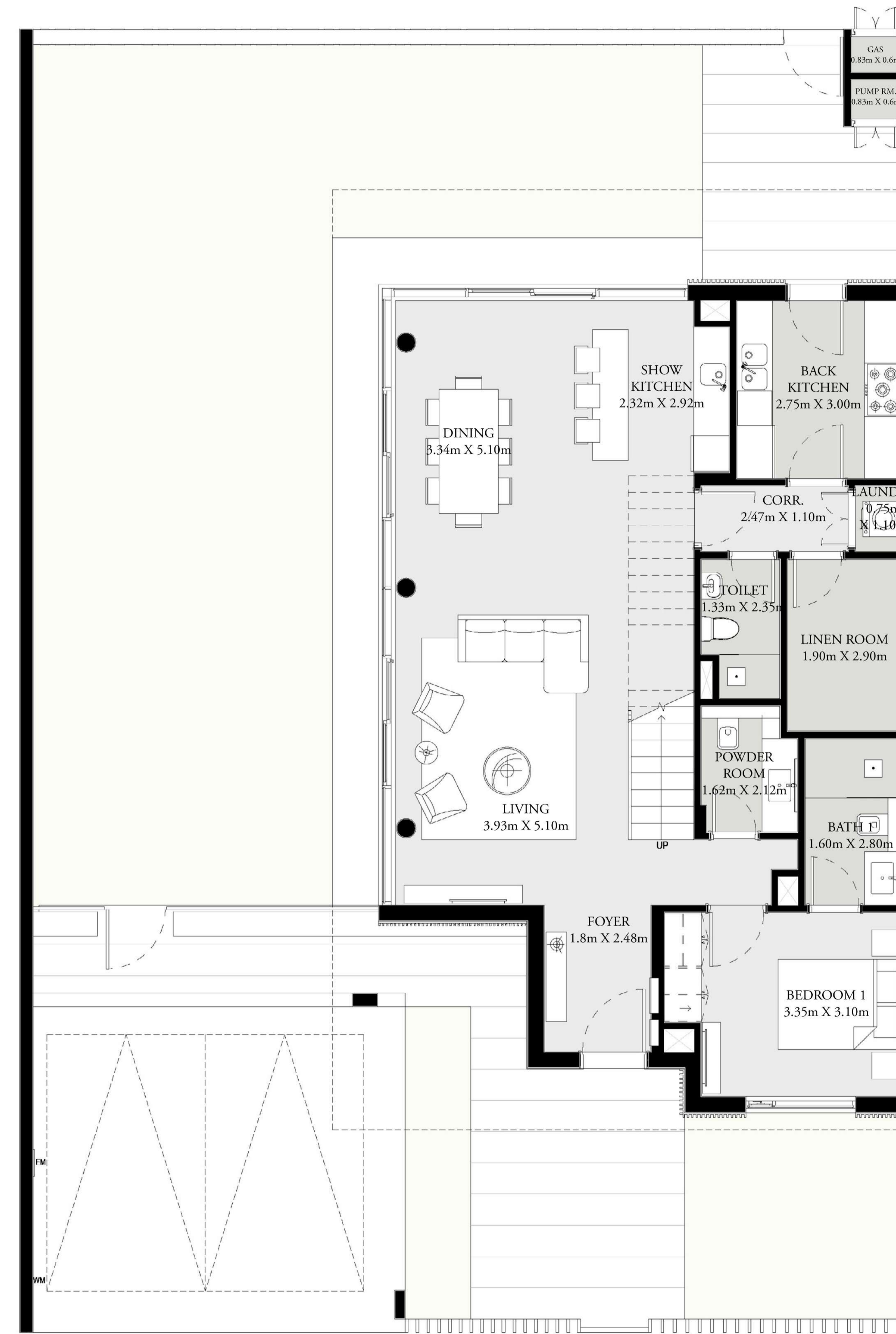
GROUND FLOOR
