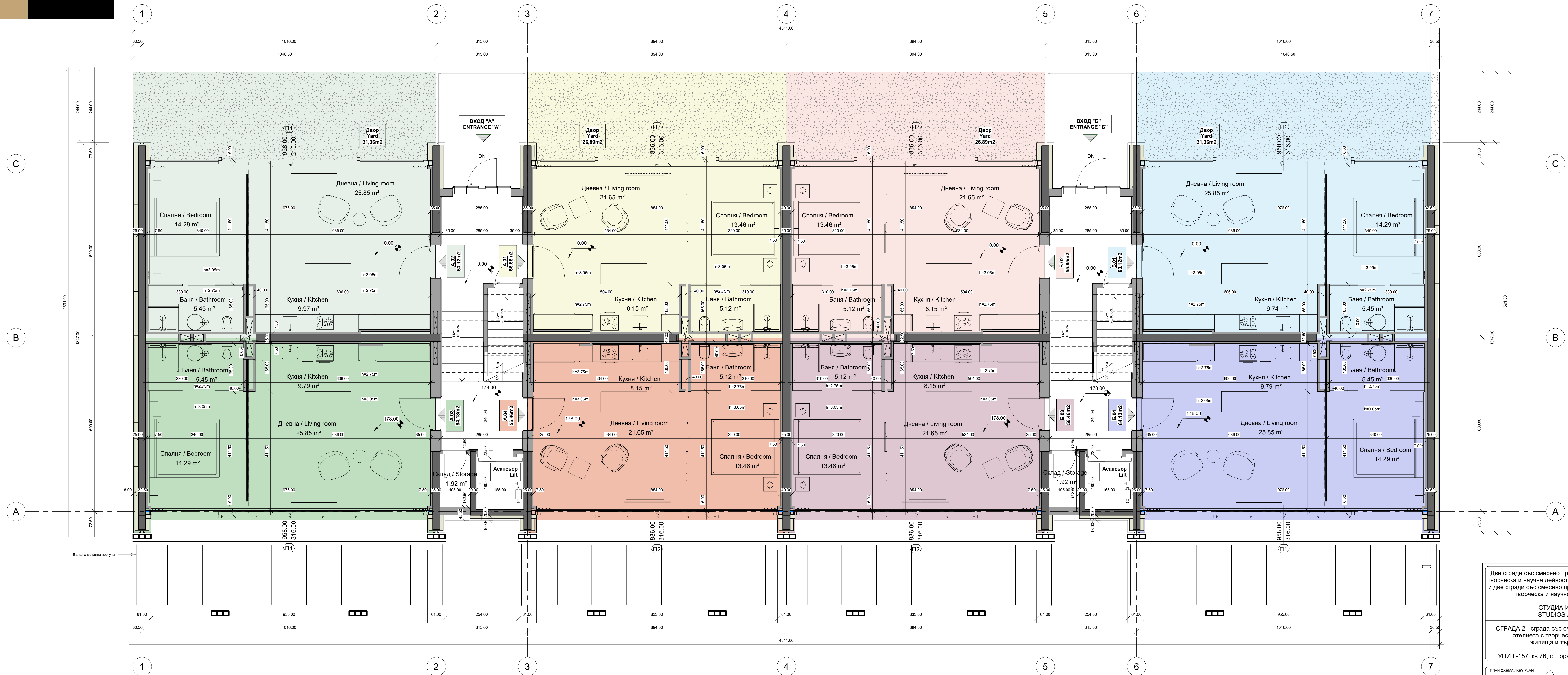
СГРАДА 2, ЕТАЖ 1 НИВО 0.00m / НИВО +1.78m BUILDING 2, FLOOR 1 LEVEL 0.00m / LEVEL +1.78m
