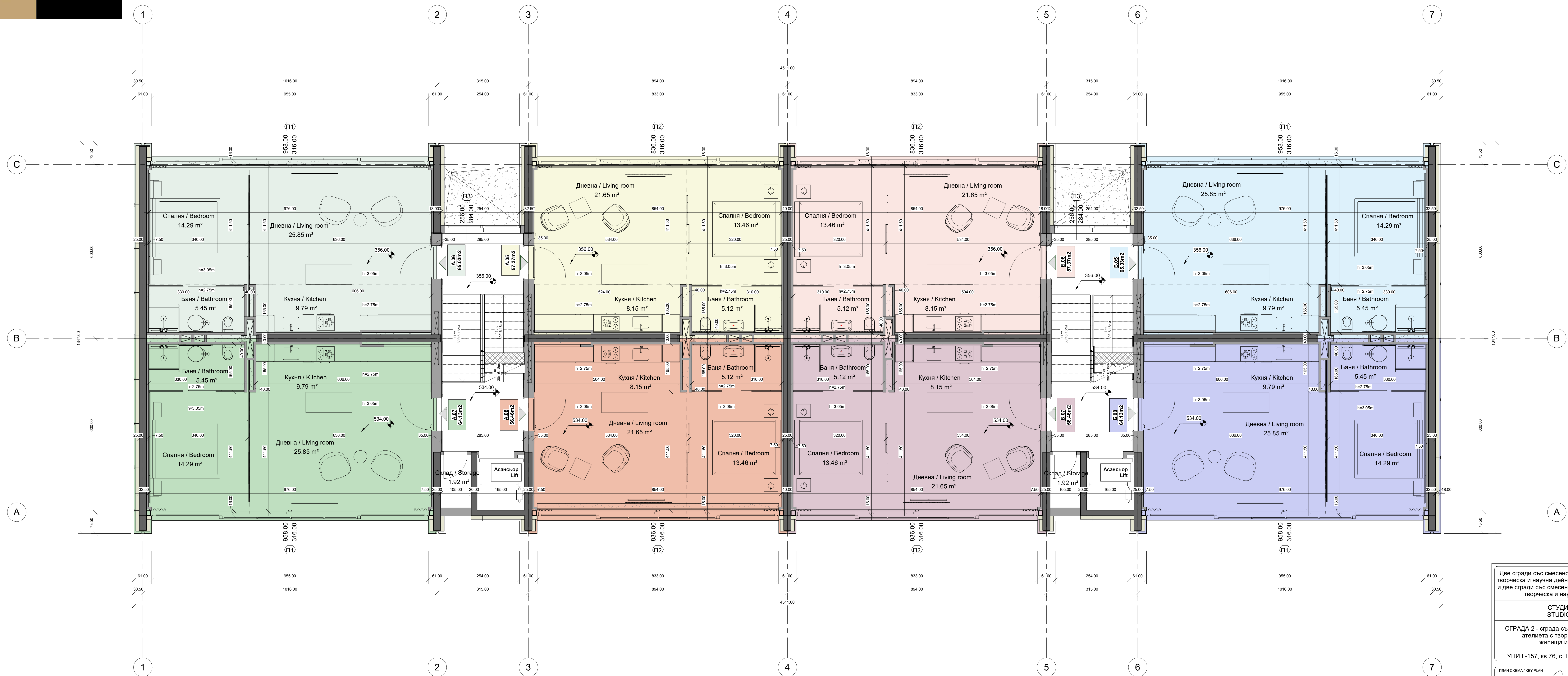
СГРАДА 2, ЕТАЖ 2 НИВО +3.56m / НИВО +5.34m BUILDING 2, FLOOR 2 LEVEL +3.56m / LEVEL +5.34m
