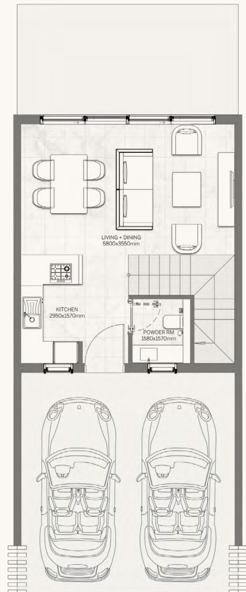
GROUND FLOOR
